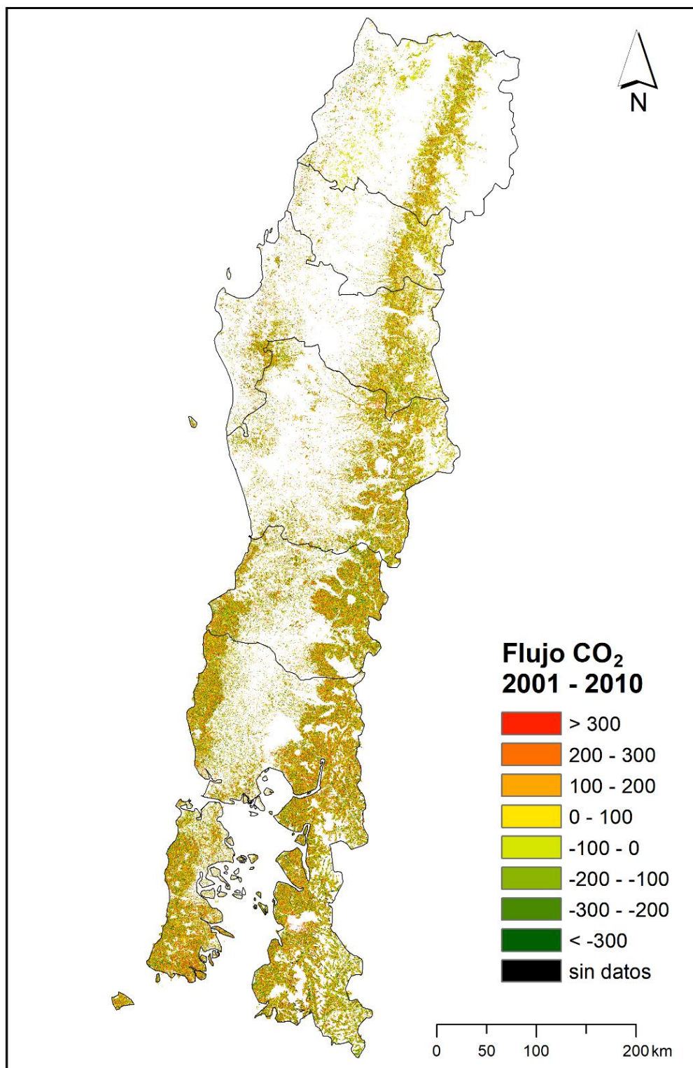
Figure 29 CO 2 flux map between 2001 and 2010 in the temperate forests of Chile.
