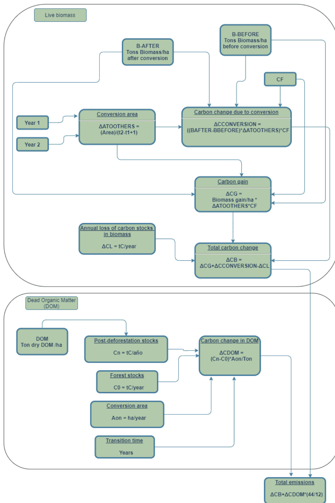
Figure 18 Step-by-step diagram for estimating emissions from deforestation.
