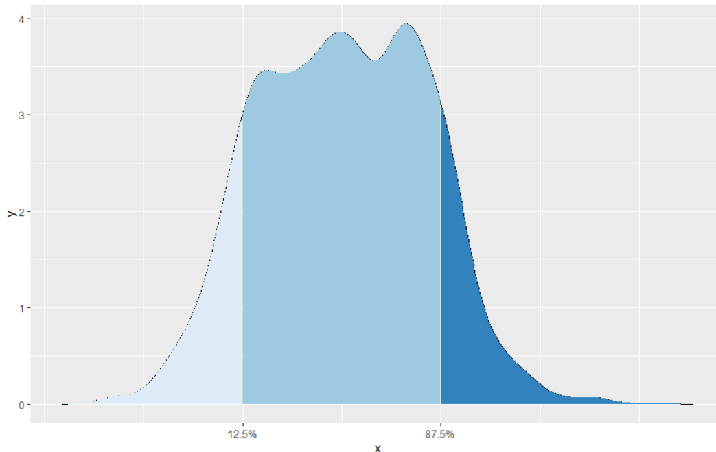
Figure 26 dNBR spectral gains histogram.
