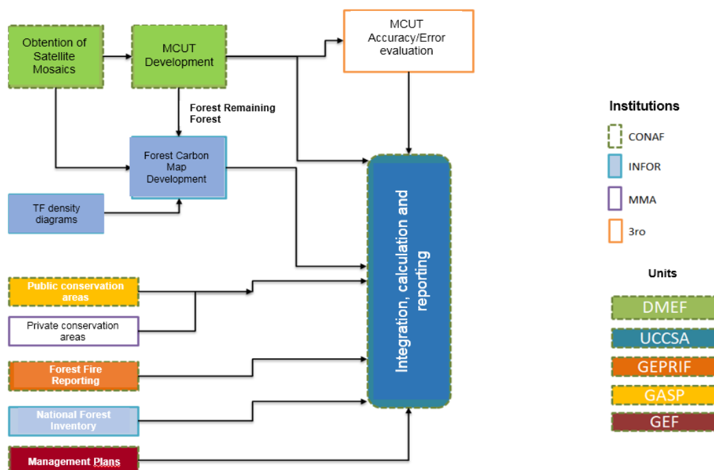
Figure 15 REDD+ reporting process general flow.
