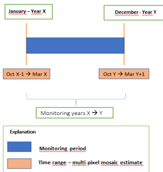
Figure 24 Example diagram for multi pixel mosaic time ranges in a monitoring period.
