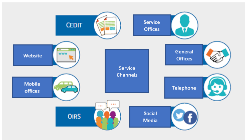
Figure 17 SIAC Service Channels (Source: CONAF, 2018).
