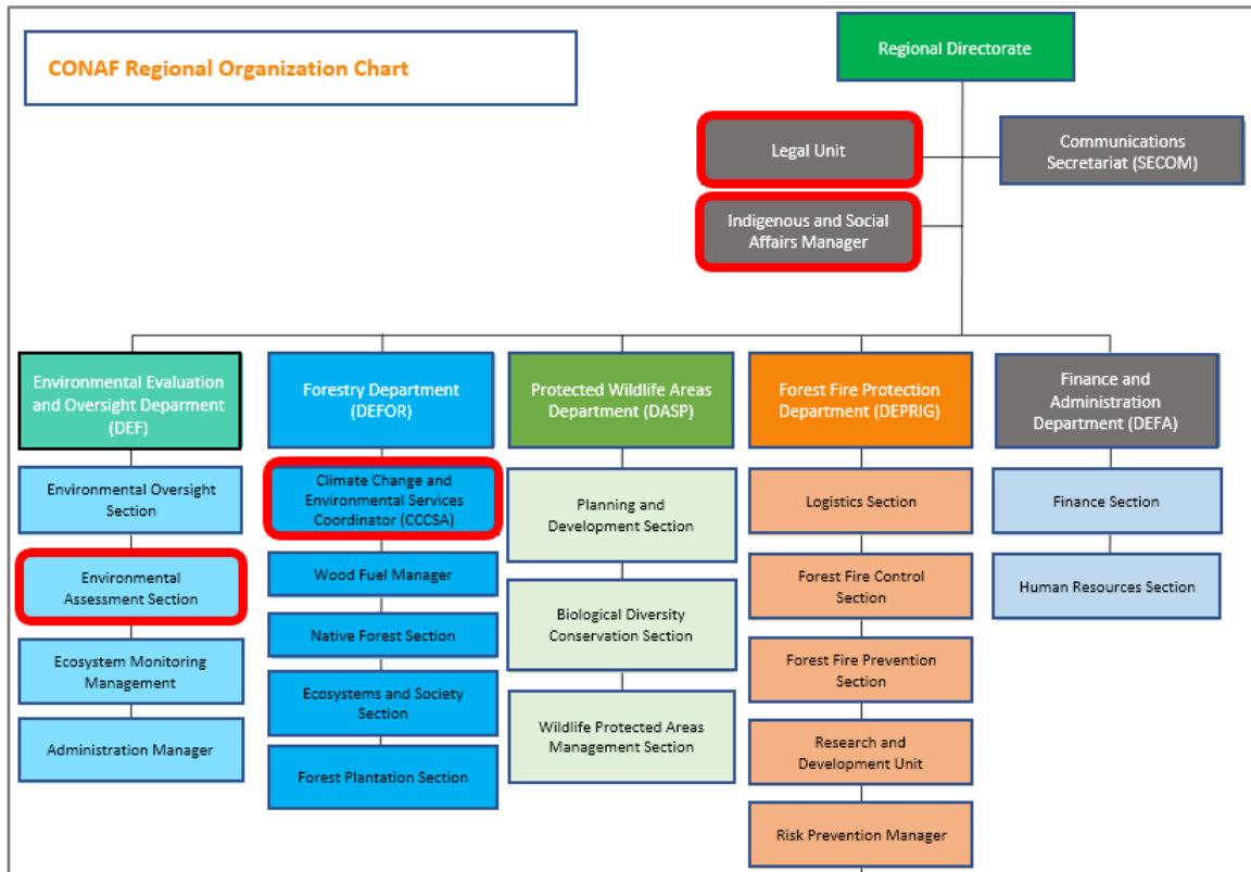
Figure 15 CONAF structure organization chart at the regional level between 2018-2019.
