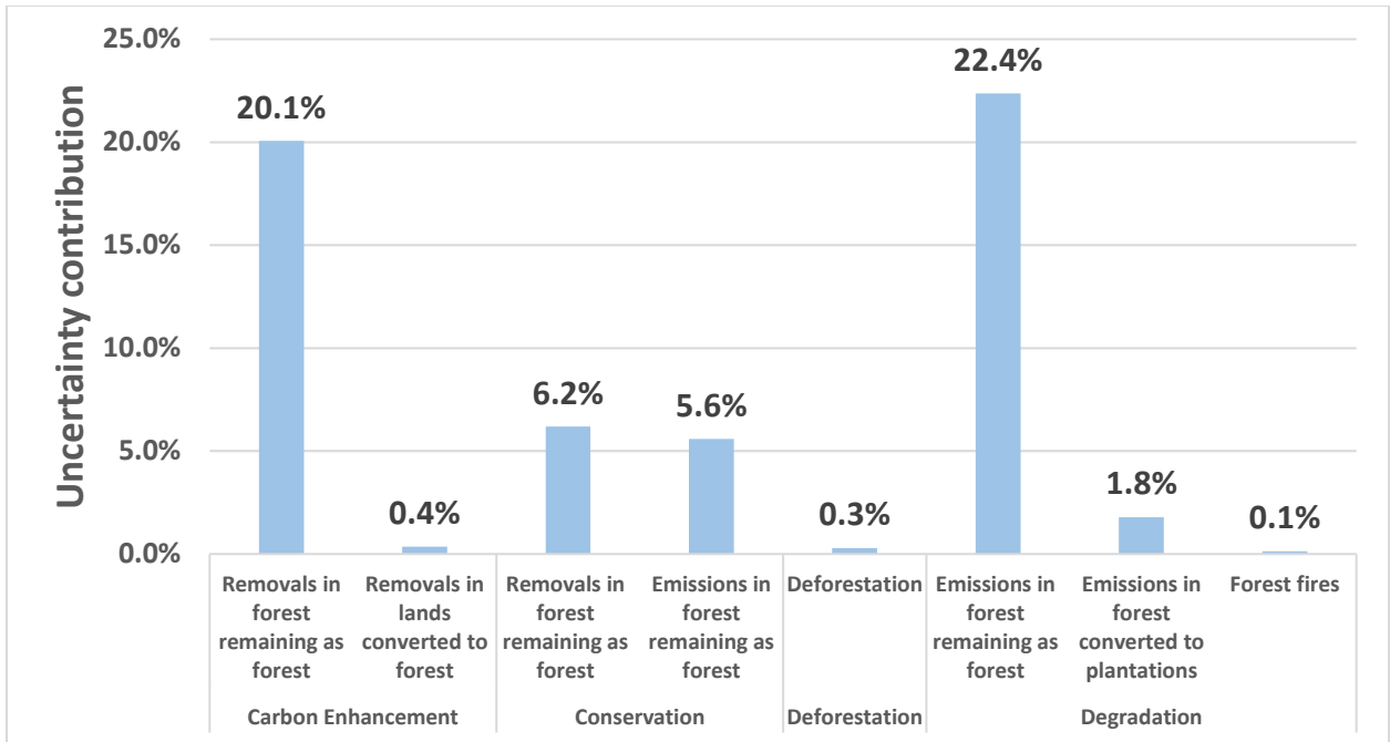
Figure 30 Results for the sensitivity analysis of ERs' global uncertainty.
