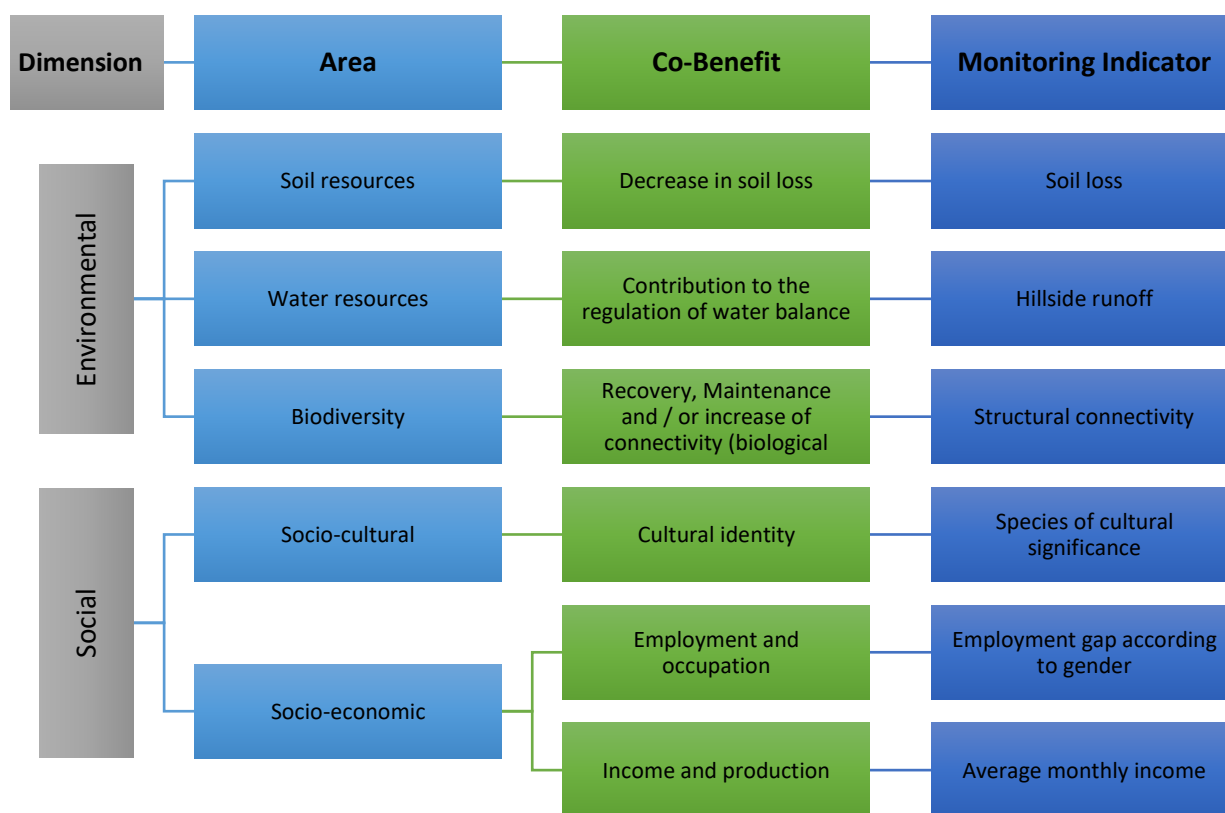
Figure 18 Selected Co-benefits and monitoring indicators (Source: Own elaboration).
