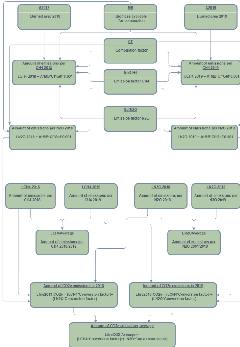
Figure 10 Step by step diagram for estimating emissions from forest fires.
