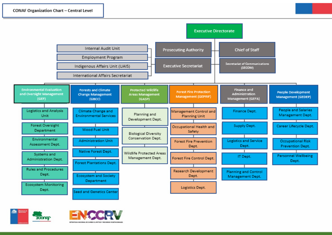
Figure 14 Central CONAF Organization Chart. Source: MGAS.
